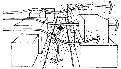
26-2. Street canyons lined with buildings of similar height, oriented perpendicular to the wind direction (top), tend to have poorer air circulation than street canyons that are lined with buildings of different heights and interspersed with open areas (bottom).
