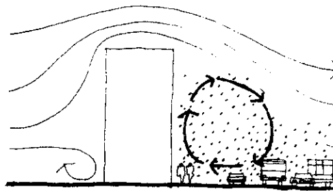
26-3. Wind shadows have reduced air circulation, and pollutants emitted with them may tend to build up.
